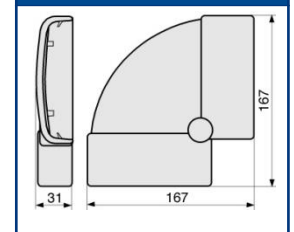
APVA Angle plat variable
